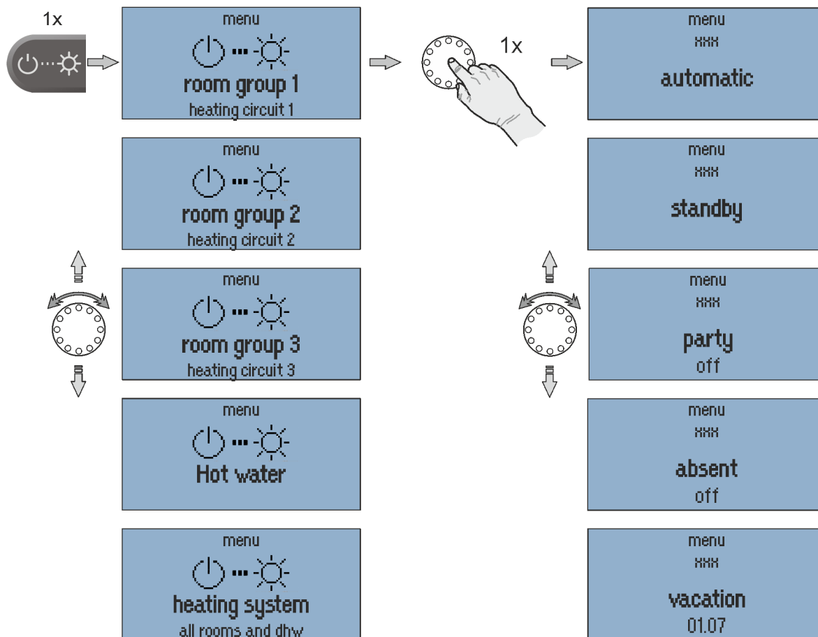
Fig. 12: Operation modes
