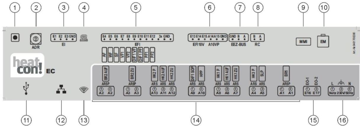
Fig. 19: heatcon! EC - connection assignment
