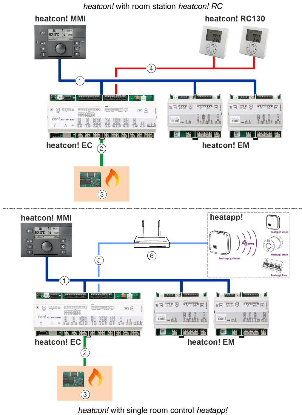
Fig. 1: heatcon! system overview
